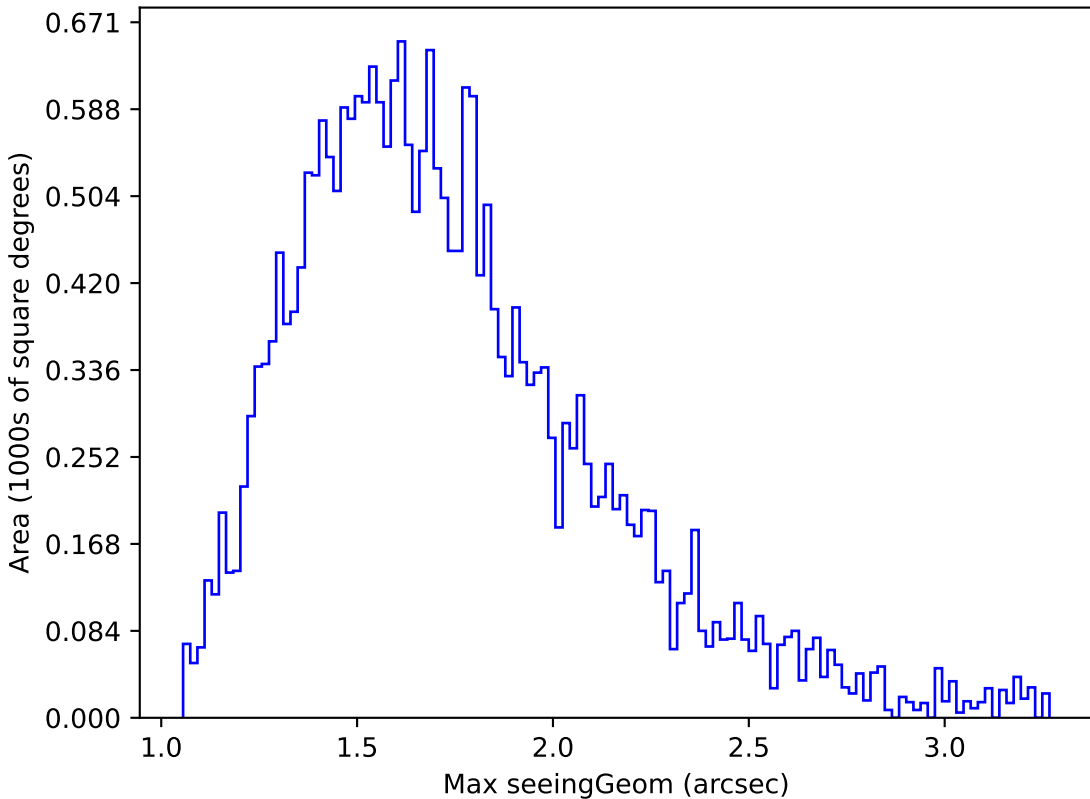
too_10_1v3.4_10yrs Yr 1 all bands: Max seeingGeom
