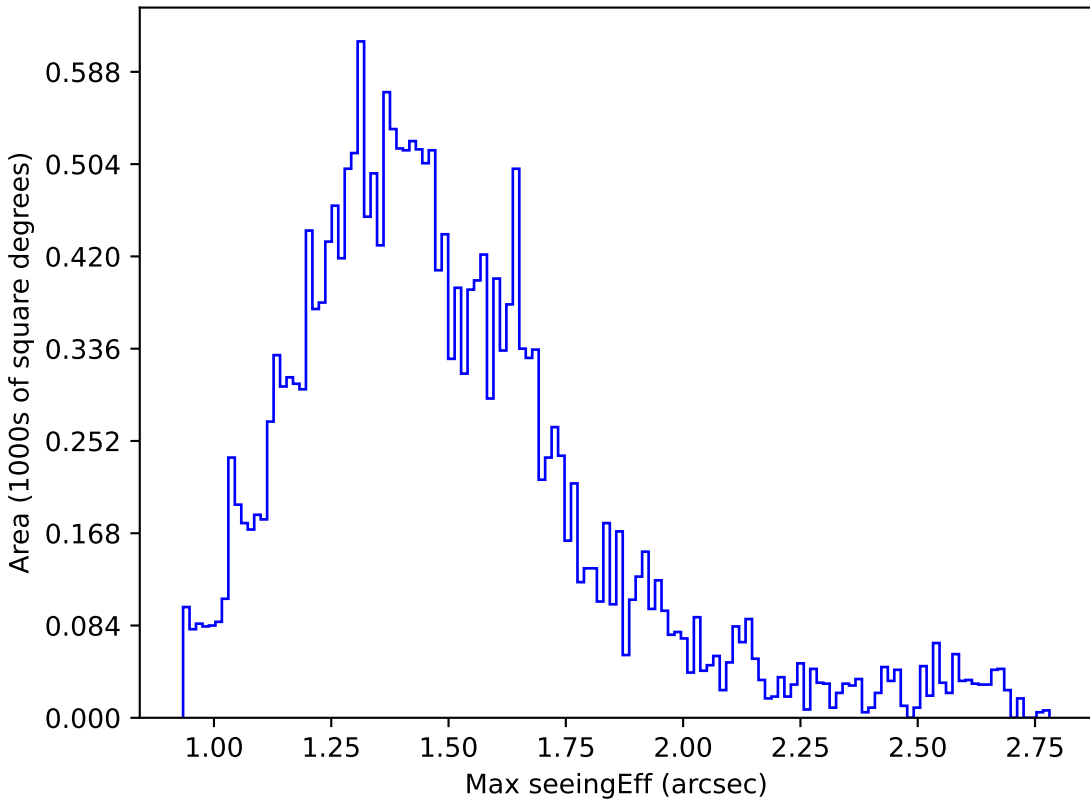
too_10_1v3.4_10yrs Yr 1 y band: Max seeingEff
