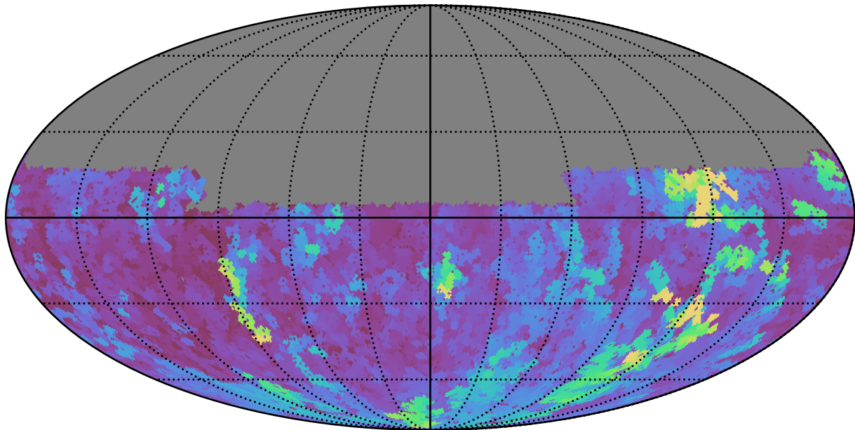
too_10_1v3.4_10yrs Yr 1 u band: Max seeingEff
