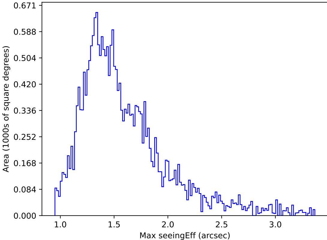
too_10_1v3.4_10yrs Yr 1 u band: Max seeingEff
