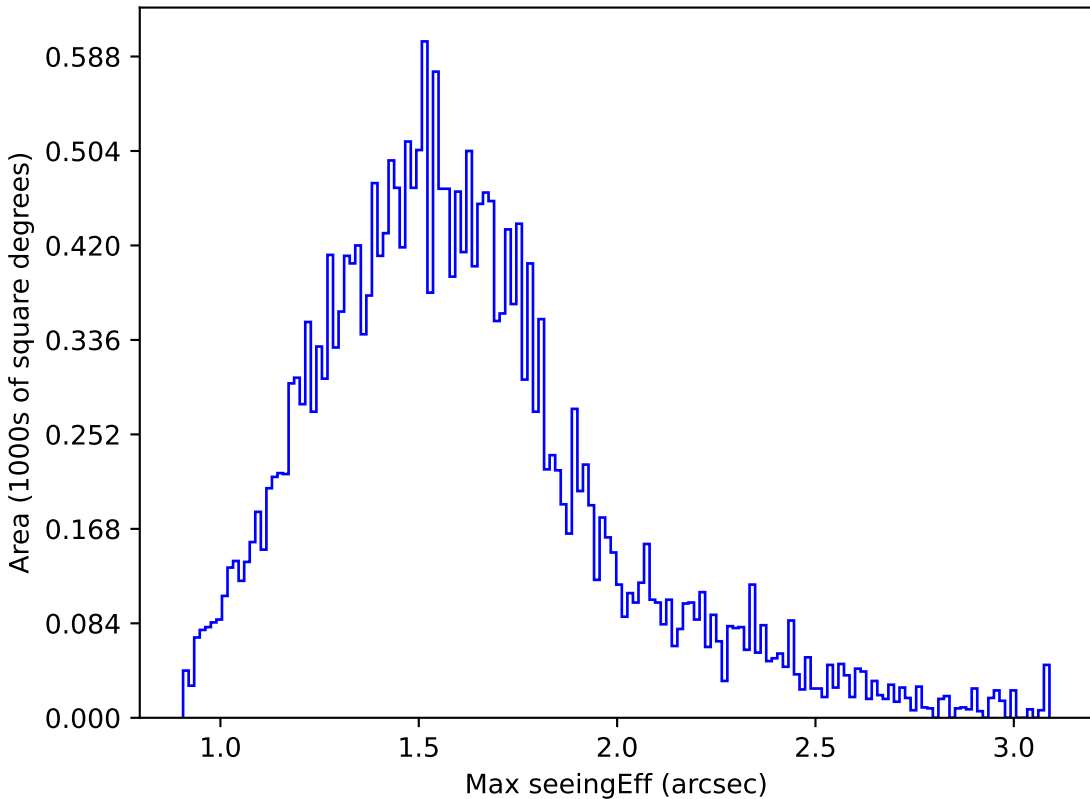
too_10_1v3.4_10yrs Yr 1 r band: Max seeingEff
