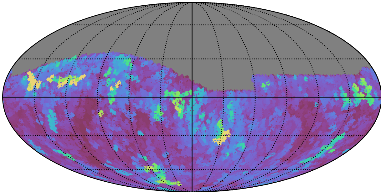
too_10_1v3.4_10yrs Yr 1 i band: Max seeingEff
