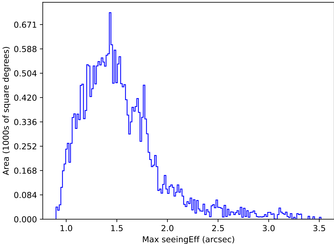
too_10_1v3.4_10yrs Yr 1 i band: Max seeingEff
