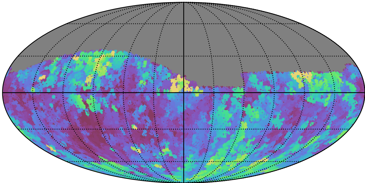
too_10_1v3.4_10yrs Yr 1 g band: Max seeingEff
