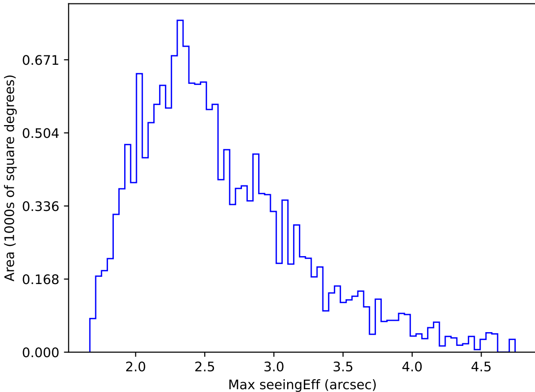
too_10_1v3.4_10yrs WFD z band: Max seeingEff
