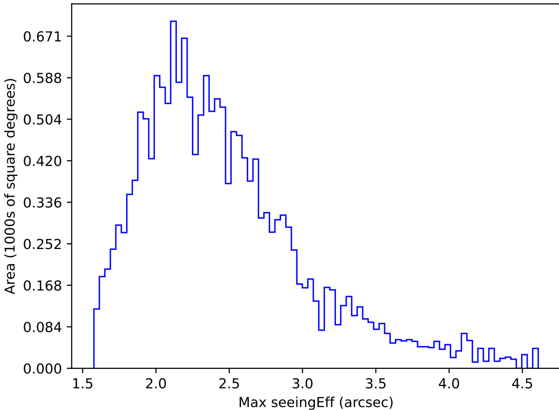
too_10_1v3.4_10yrs WFD y band: Max seeingEff
