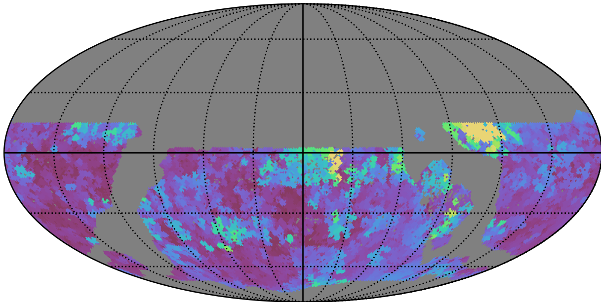
too_10_1v3.4_10yrs WFD u band: Max seeingEff
