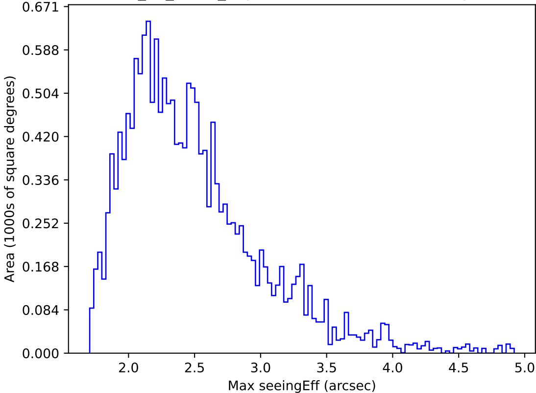
too_10_1v3.4_10yrs WFD u band: Max seeingEff
