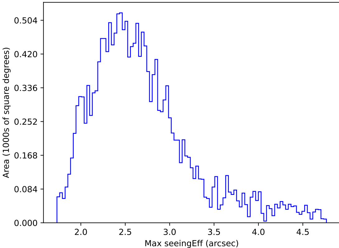
too_10_1v3.4_10yrs WFD r band: Max seeingEff
