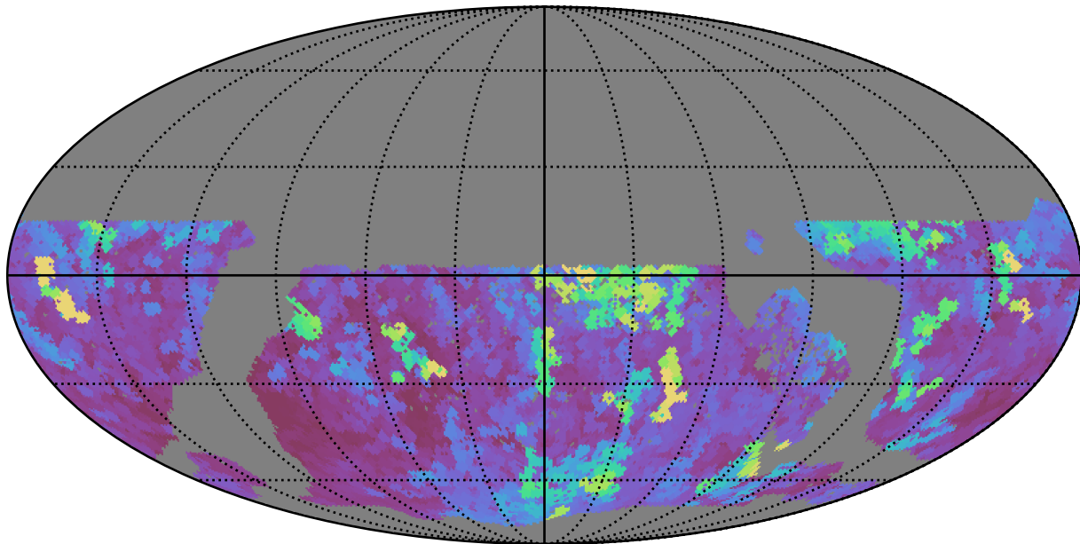
too_10_1v3.4_10yrs WFD i band: Max seeingEff
