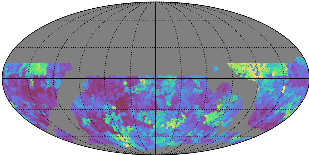
too_10_1v3.4_10yrs WFD g band: Max seeingEff
