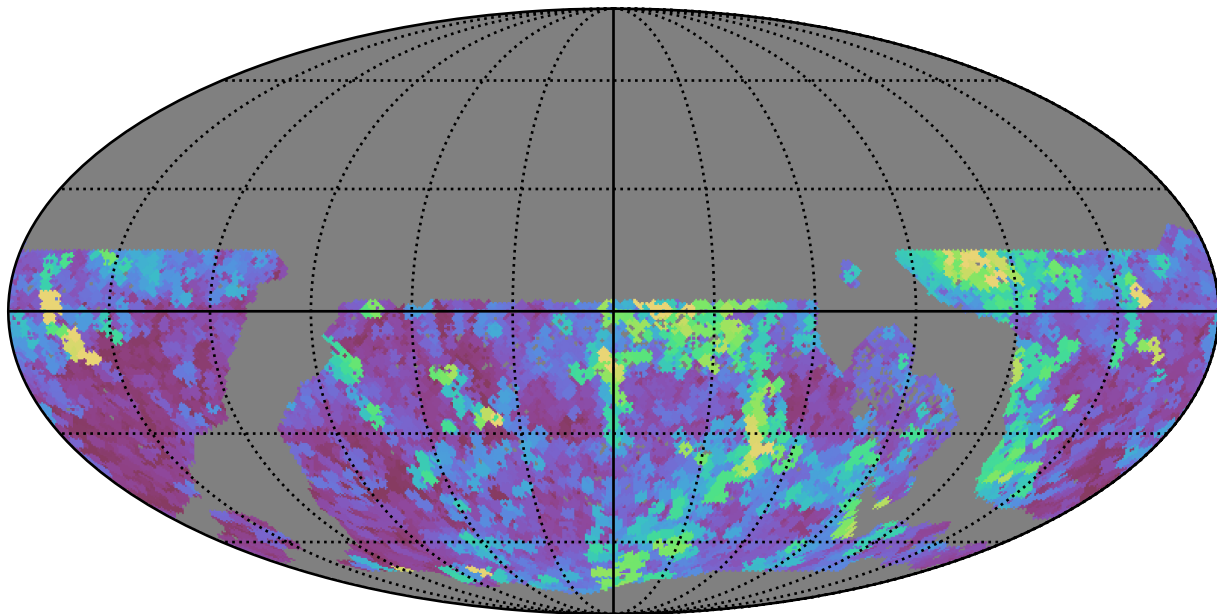
too_10_1v3.4_10yrs WFD all bands: Max seeingEff
