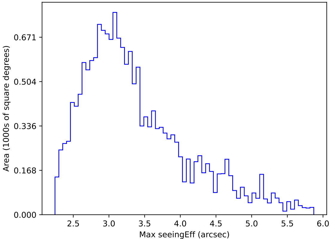
too_10_1v3.4_10yrs WFD all bands: Max seeingEff
