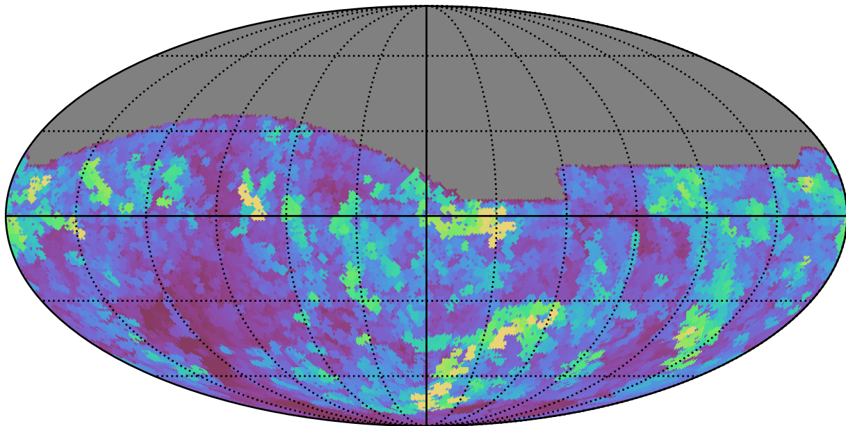
too_10_1v3.4_10yrs All sky z band: Max seeingEff
