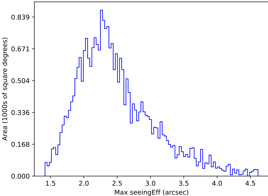
too_10_1v3.4_10yrs All sky z band: Max seeingEff
