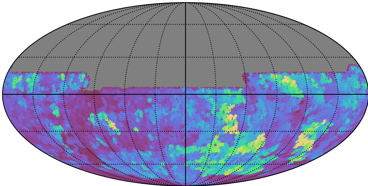
too_10_1v3.4_10yrs All sky y band: Max seeingEff
