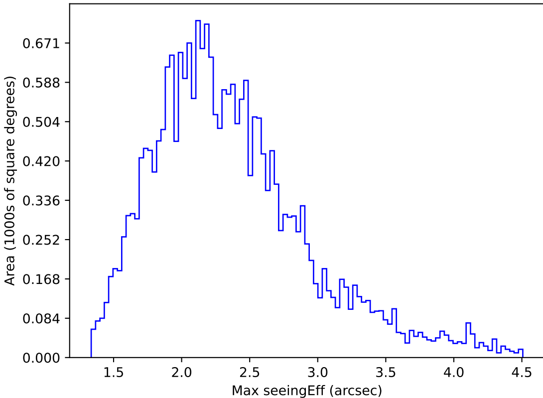
too_10_1v3.4_10yrs All sky y band: Max seeingEff
