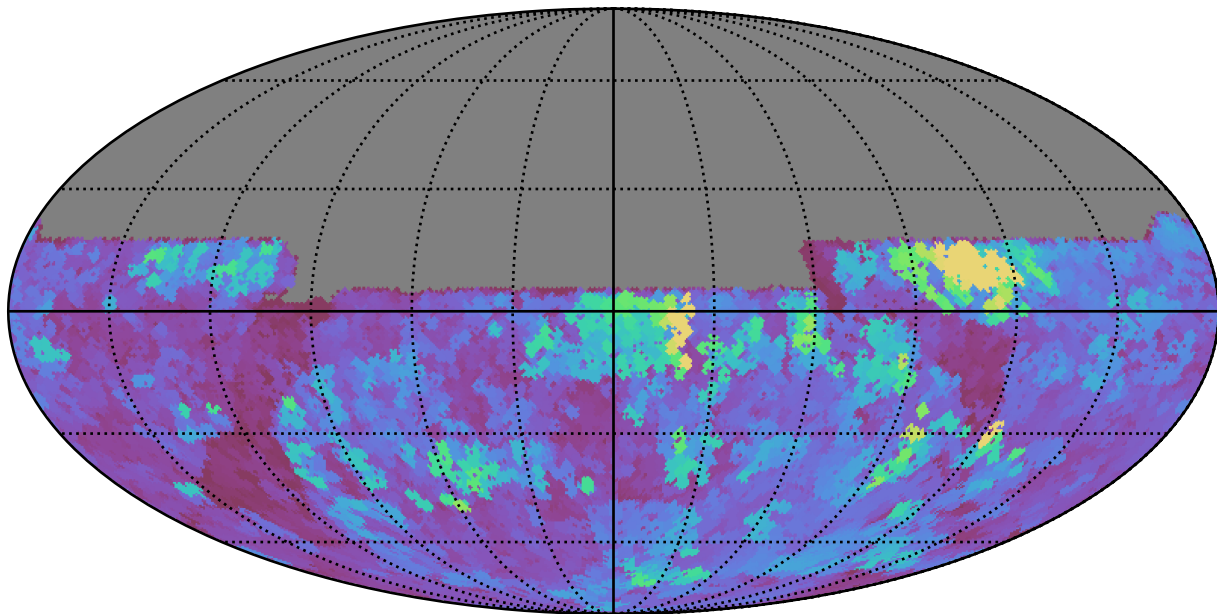
too_10_1v3.4_10yrs All sky u band: Max seeingEff
