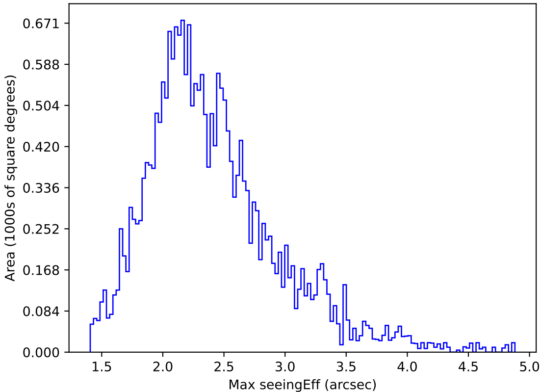
too_10_1v3.4_10yrs All sky u band: Max seeingEff
