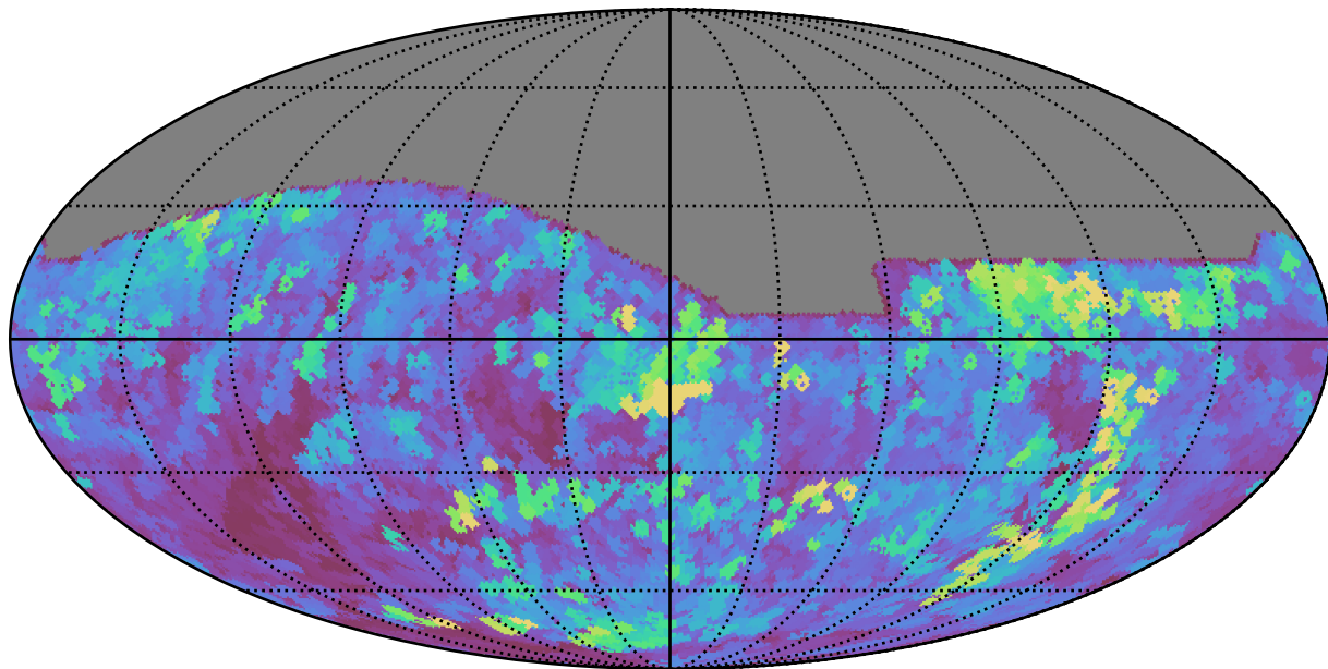
too_10_1v3.4_10yrs All sky r band: Max seeingEff
