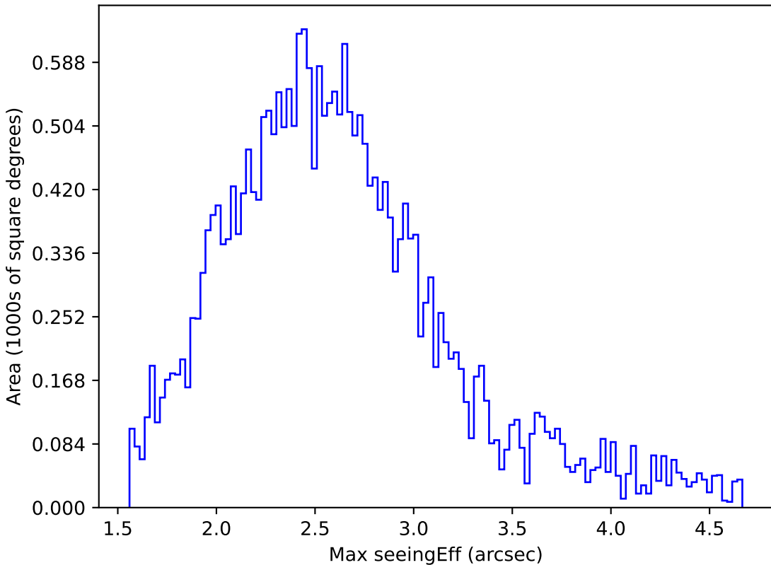
too_10_1v3.4_10yrs All sky r band: Max seeingEff
