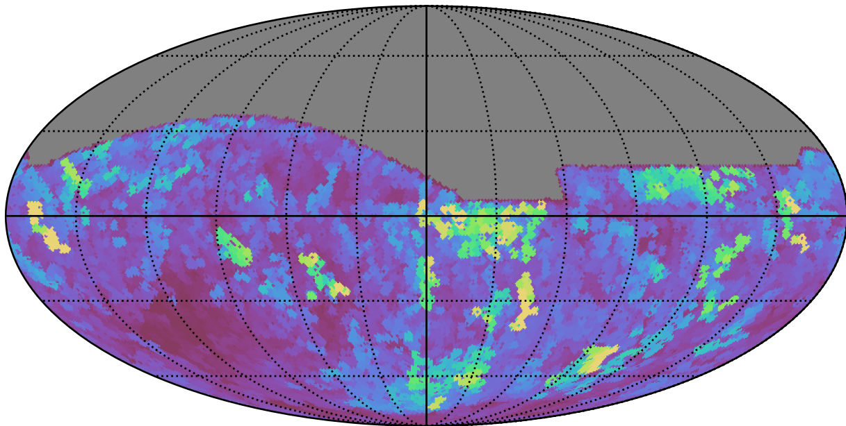
too_10_1v3.4_10yrs All sky i band: Max seeingEff
