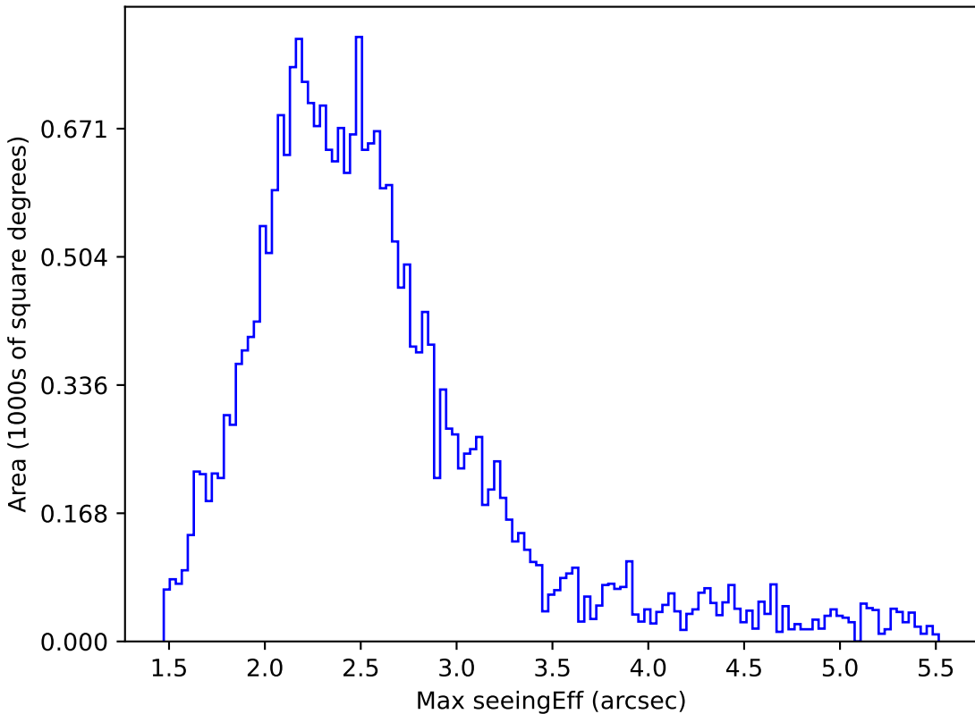
too_10_1v3.4_10yrs All sky i band: Max seeingEff
