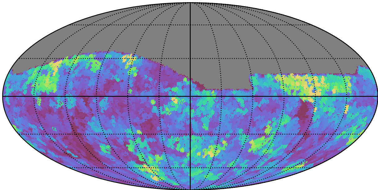
too_10_1v3.4_10yrs All sky g band: Max seeingEff
