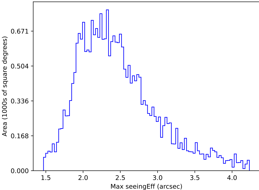
too_10_1v3.4_10yrs All sky g band: Max seeingEff
