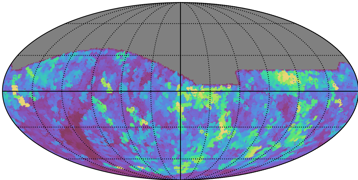
too_10_1v3.4_10yrs All sky all bands: Max seeingEff
