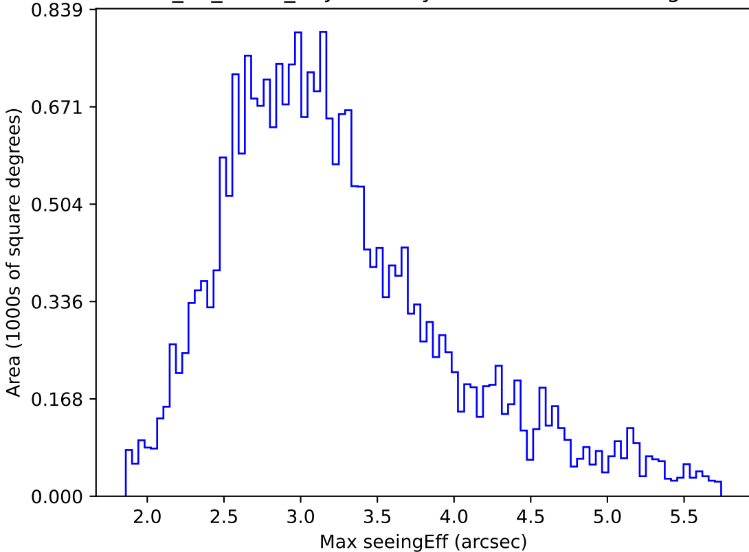
too_10_1v3.4_10yrs All sky all bands: Max seeingEff
