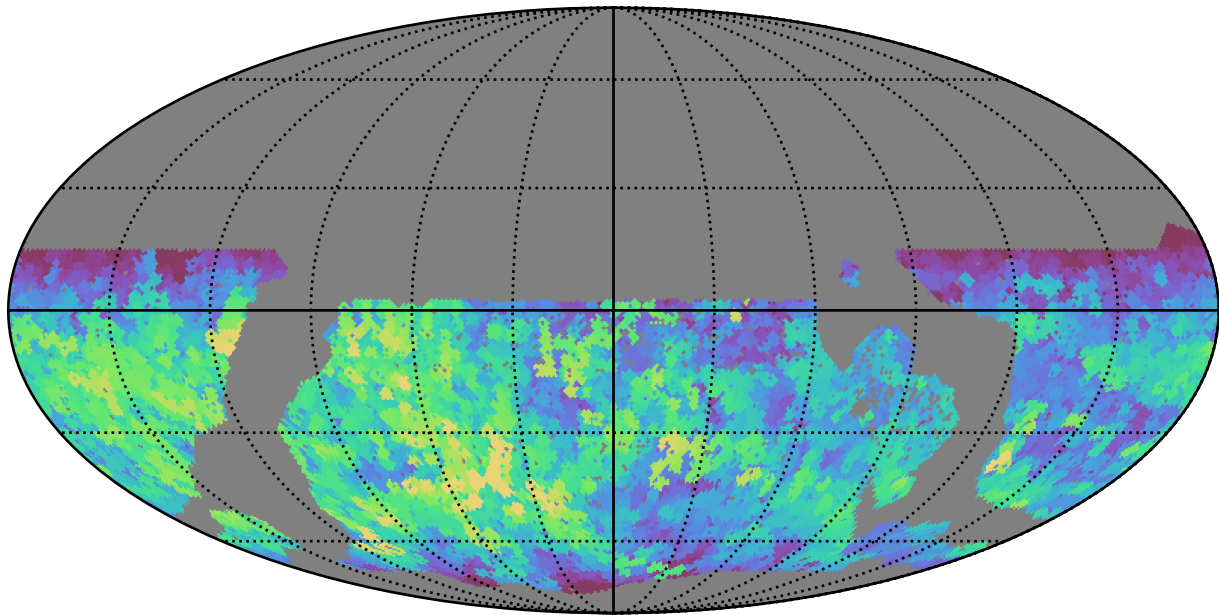
too_10_1v3.4_10yrs WFD z band: Max saturation_mag
