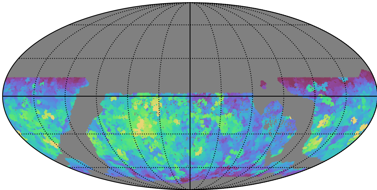
too_10_1v3.4_10yrs WFD r band: Max saturation_mag
