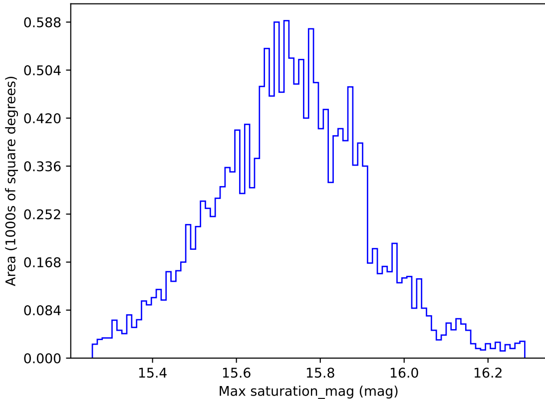
too_10_1v3.4_10yrs WFD g band: Max saturation_mag
