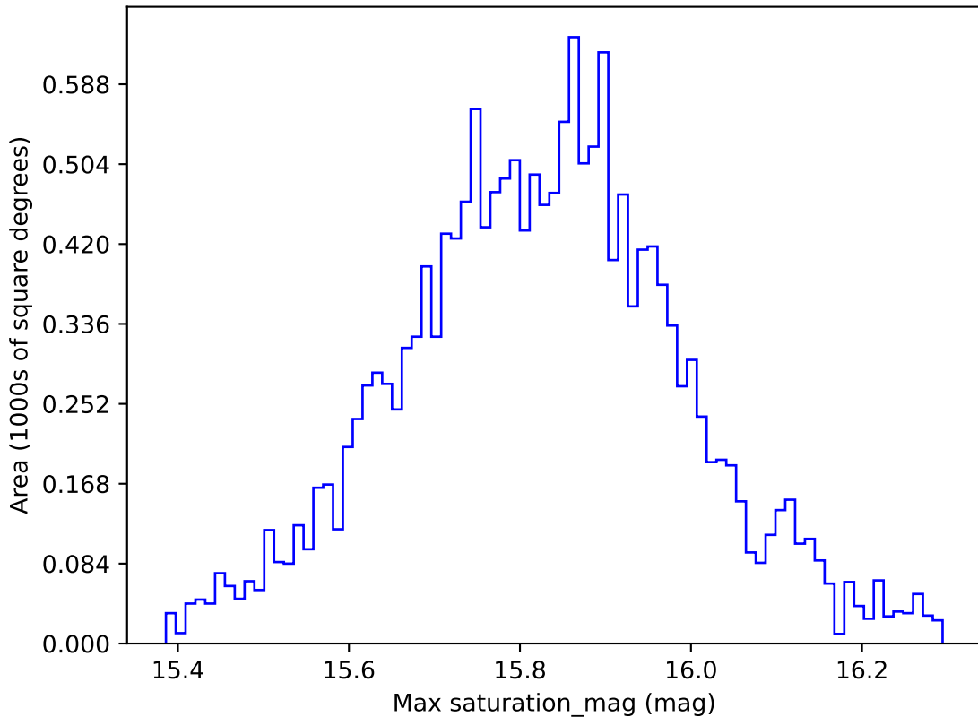
too_10_1v3.4_10yrs WFD all bands: Max saturation_mag
