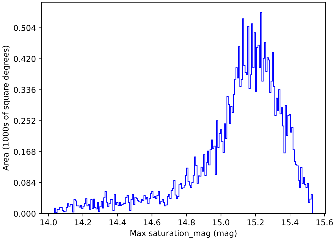
too_10_1v3.4_10yrs All sky z band: Max saturation_mag
