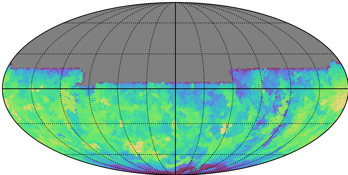
too_10_1v3.4_10yrs All sky u band: Max saturation_mag
