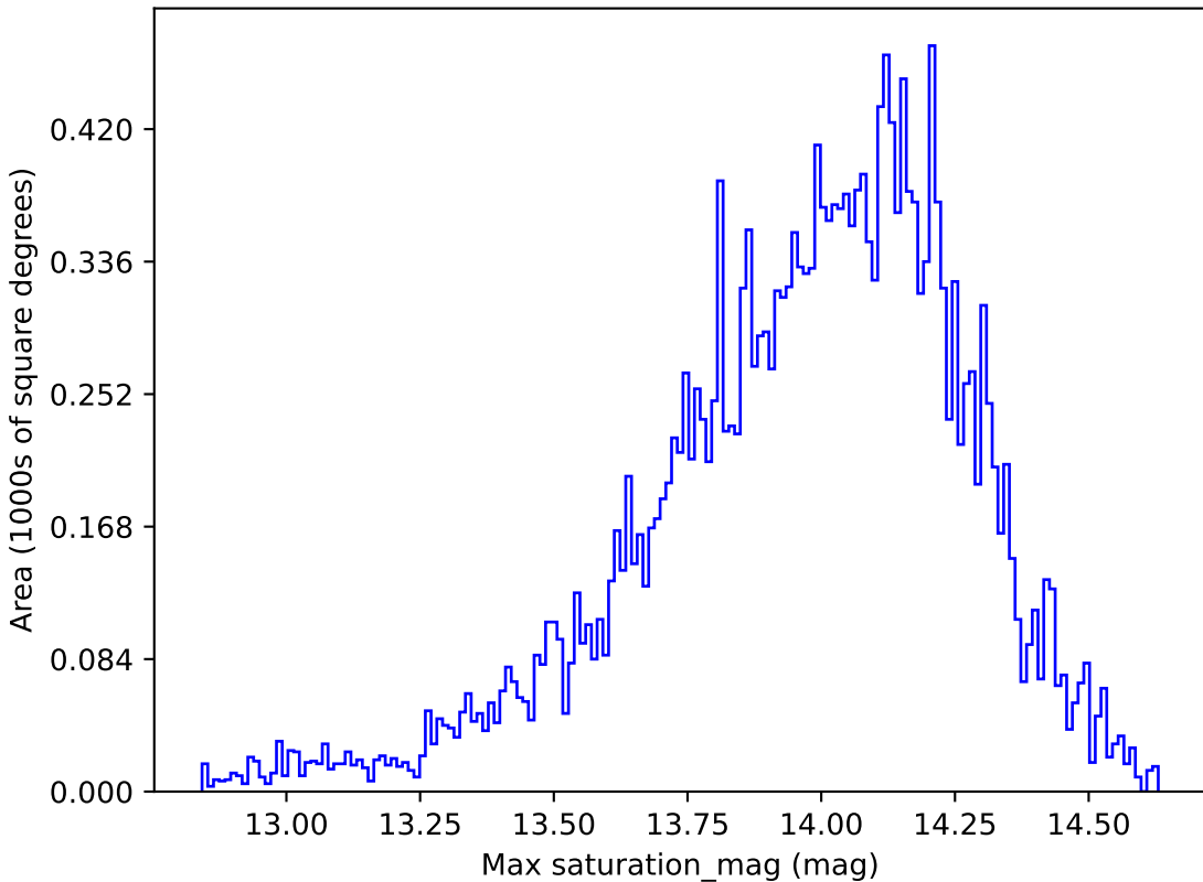
too_10_1v3.4_10yrs All sky u band: Max saturation_mag
