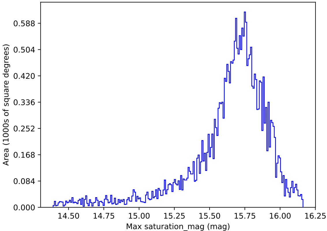
too_10_1v3.4_10yrs All sky r band: Max saturation_mag
