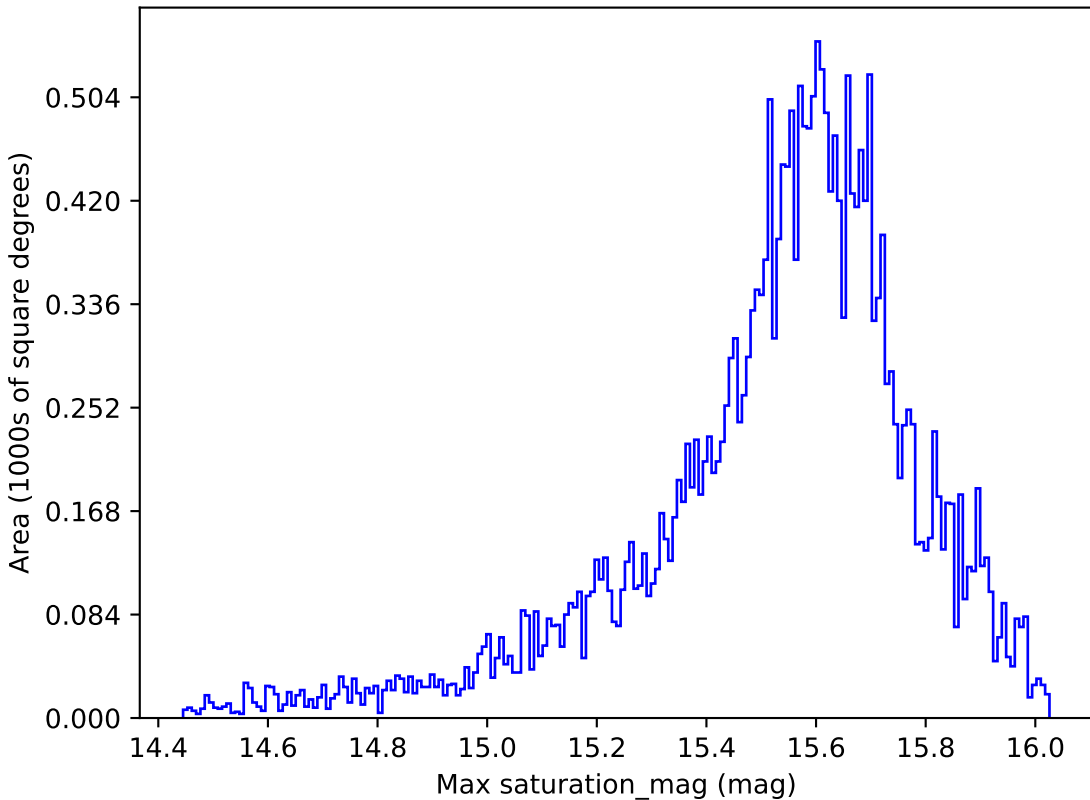
too_10_1v3.4_10yrs All sky i band: Max saturation_mag
