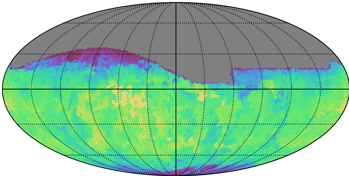
too_10_1v3.4_10yrs All sky g band: Max saturation_mag
