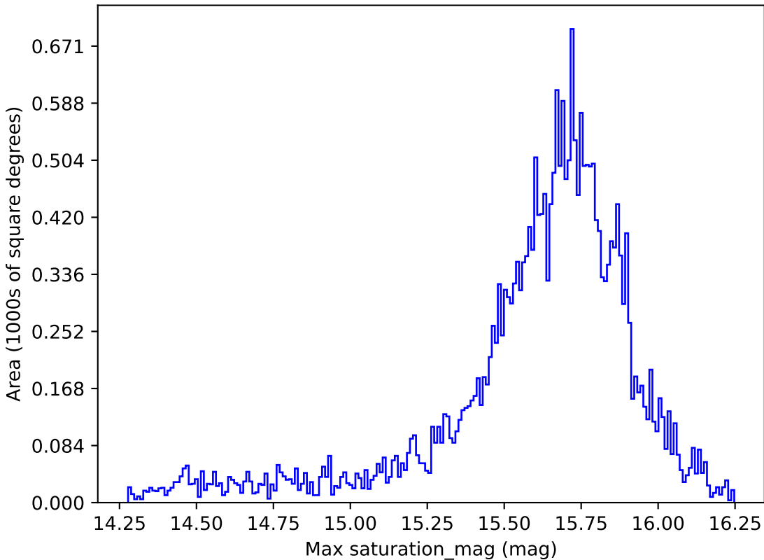
too_10_1v3.4_10yrs All sky g band: Max saturation_mag
