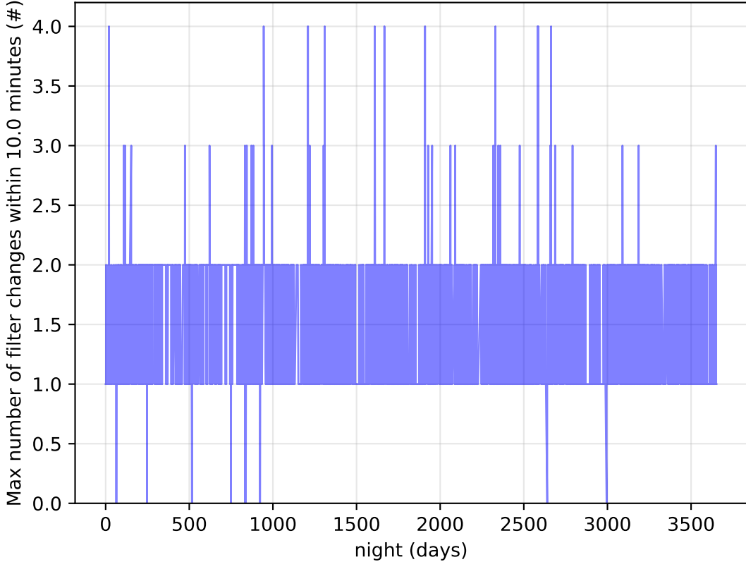
too_10_1v3.4_10yrs Per Night: Max number of filter changes within 10.0 minutes
