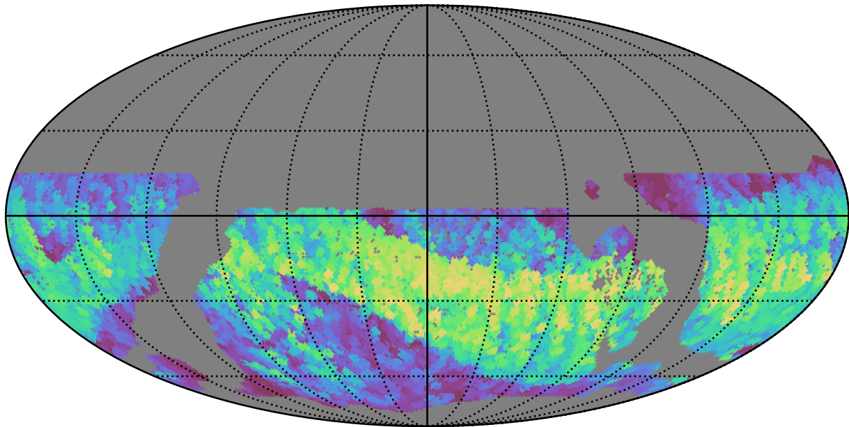
too_10_1v3.4_10yrs WFD z band: Max normairmass
