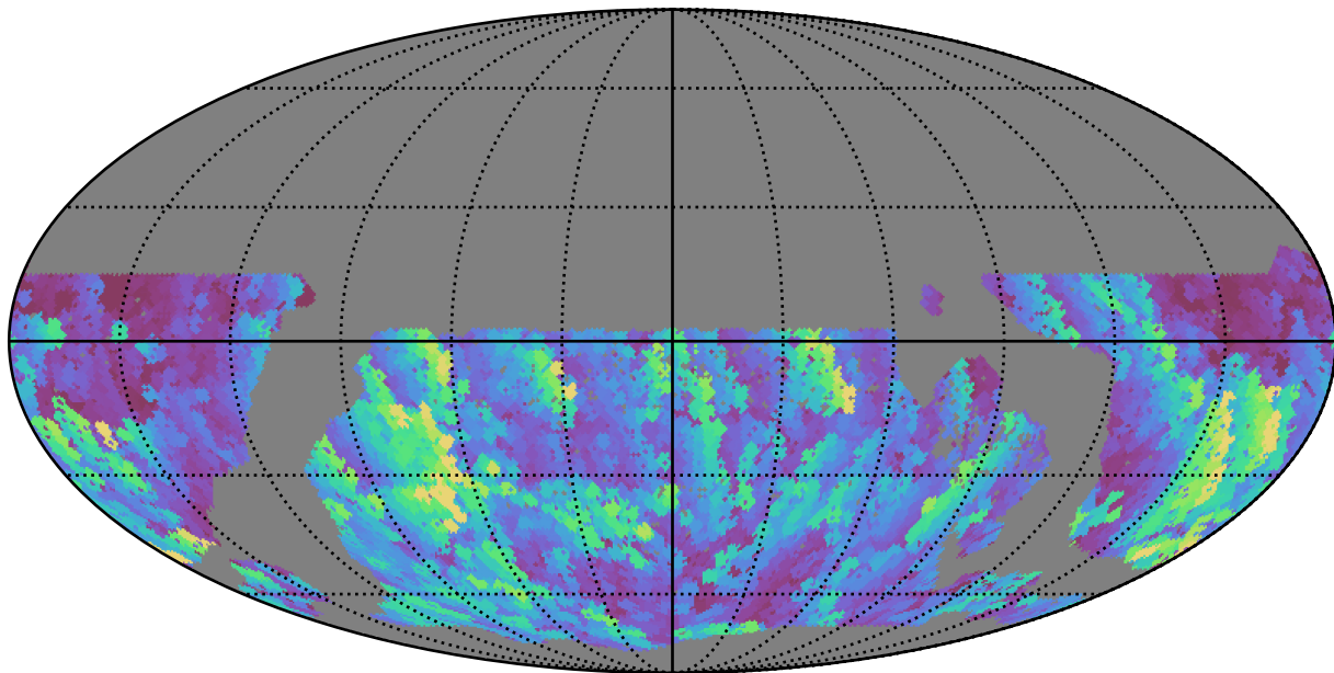
too_10_1v3.4_10yrs WFD u band: Max normairmass
