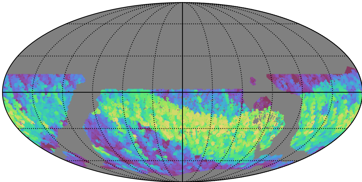
too_10_1v3.4_10yrs WFD i band: Max normairmass
