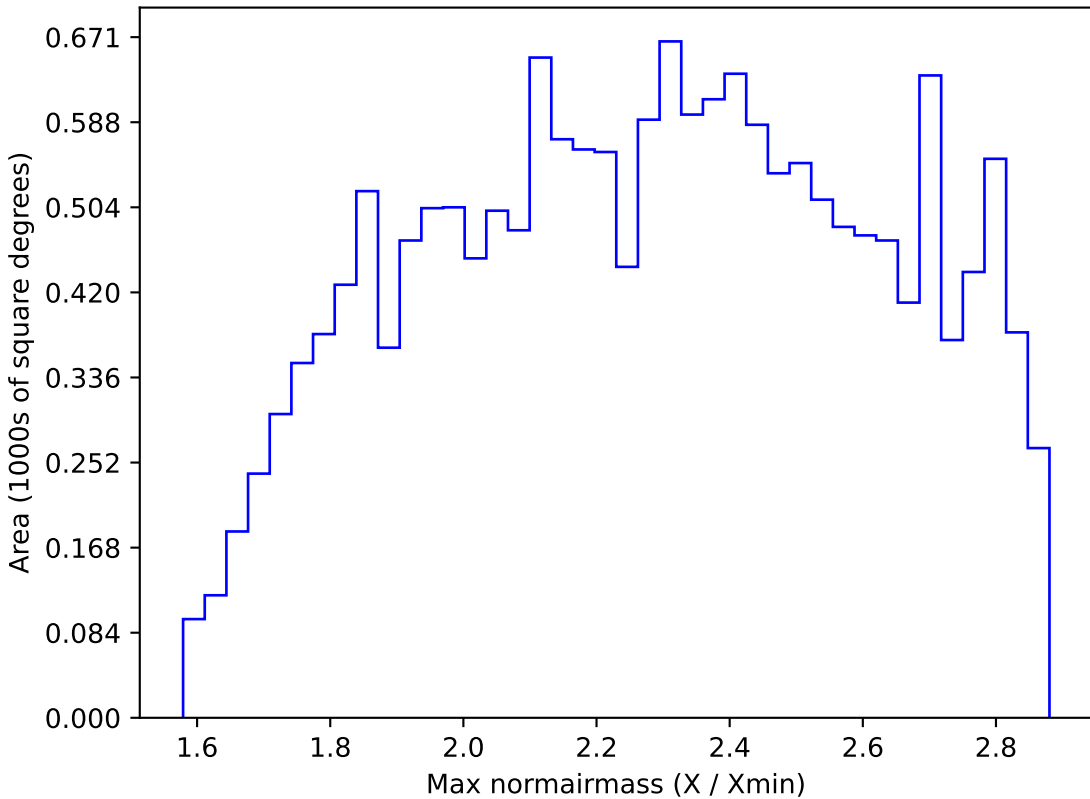
too_10_1v3.4_10yrs WFD i band: Max normairmass
