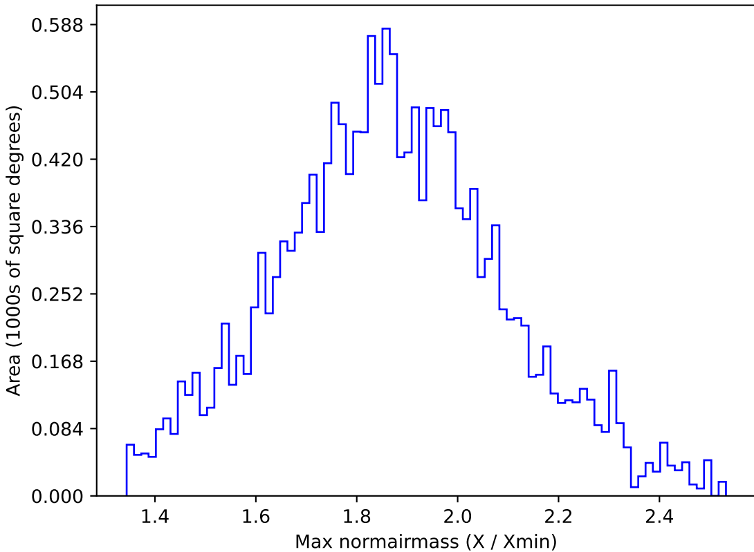
too_10_1v3.4_10yrs WFD g band: Max normairmass
