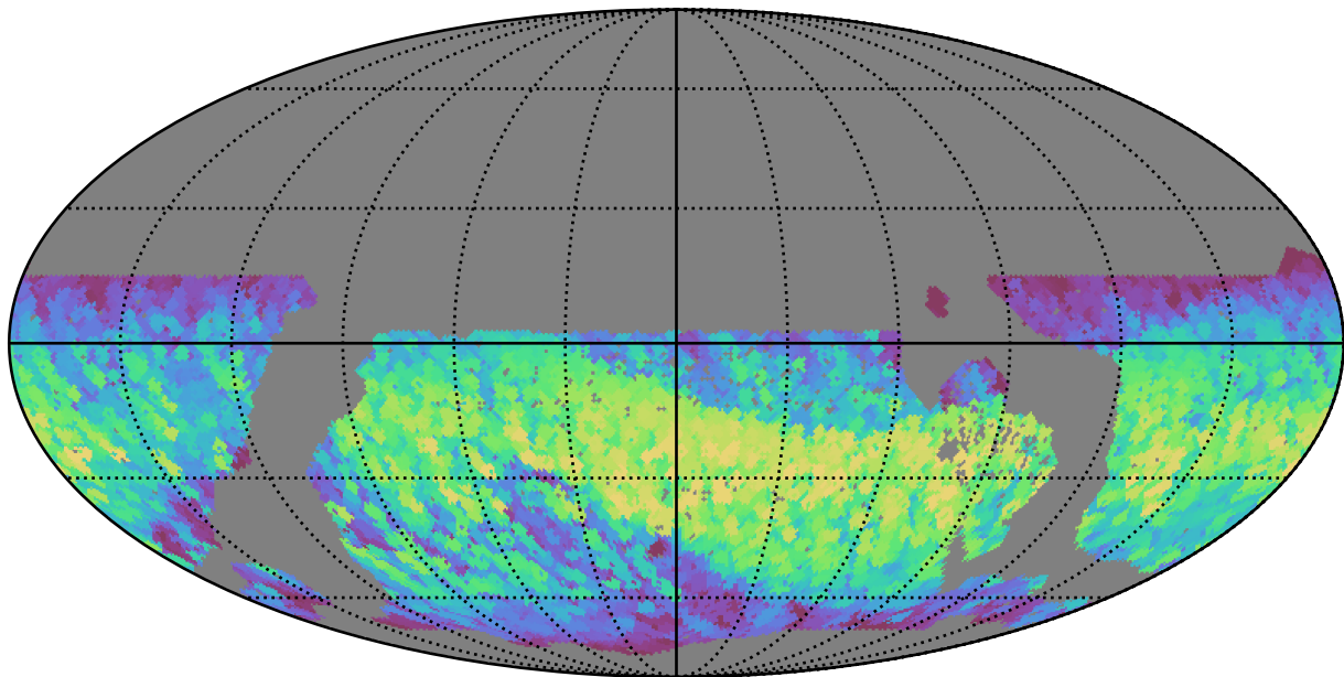
too_10_1v3.4_10yrs WFD all bands: Max normairmass
