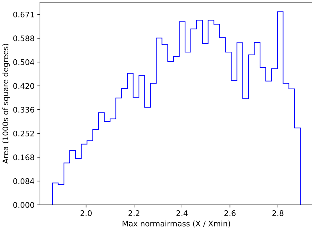
too_10_1v3.4_10yrs WFD all bands: Max normairmass
